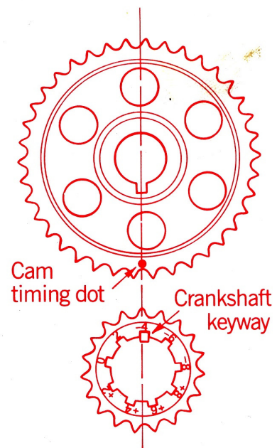
Retard 4° as drawn
