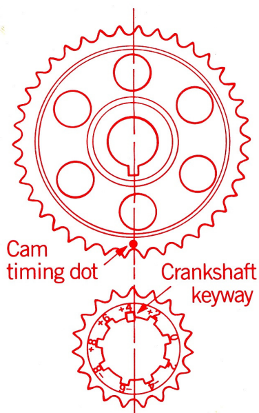
Advanced 4° as drawn
